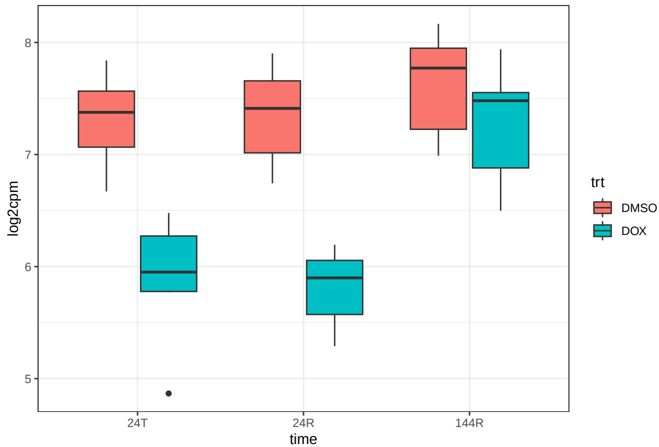
gene 26037 SIPA1L1 dist 32767
